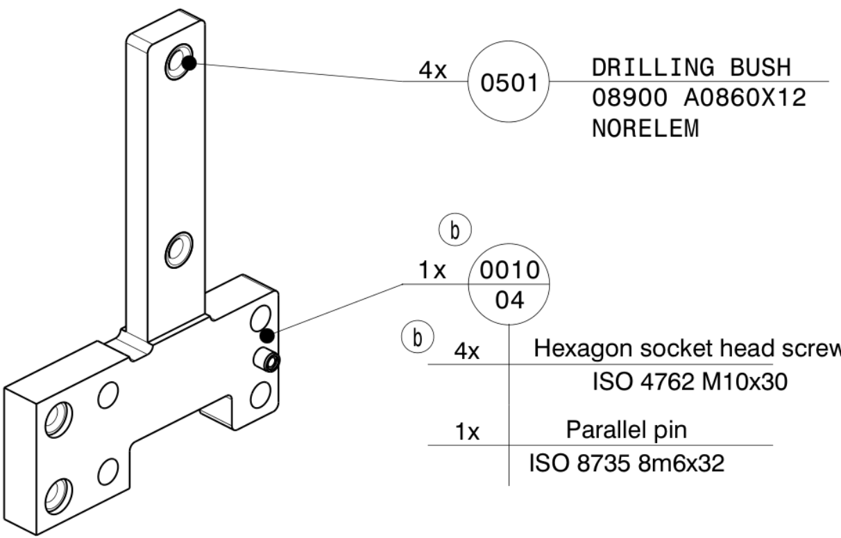
Isometric view Scale: 1:2
