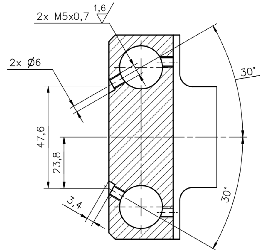
A – A (1 : 1)
